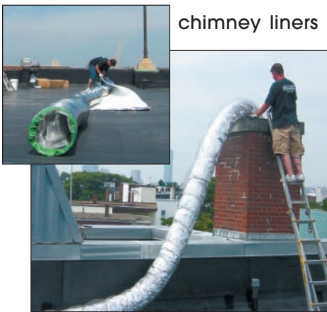
Blanket insulation must be carefully installed.
